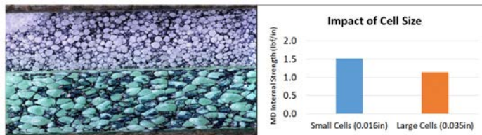
Figure 7: Cell size comparison of 2 pcf 1/8” thick LDPE foam. Top: 0.016” Bottom: 0.035”
